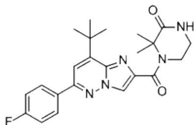
PC-6208801, DMSO-d6
